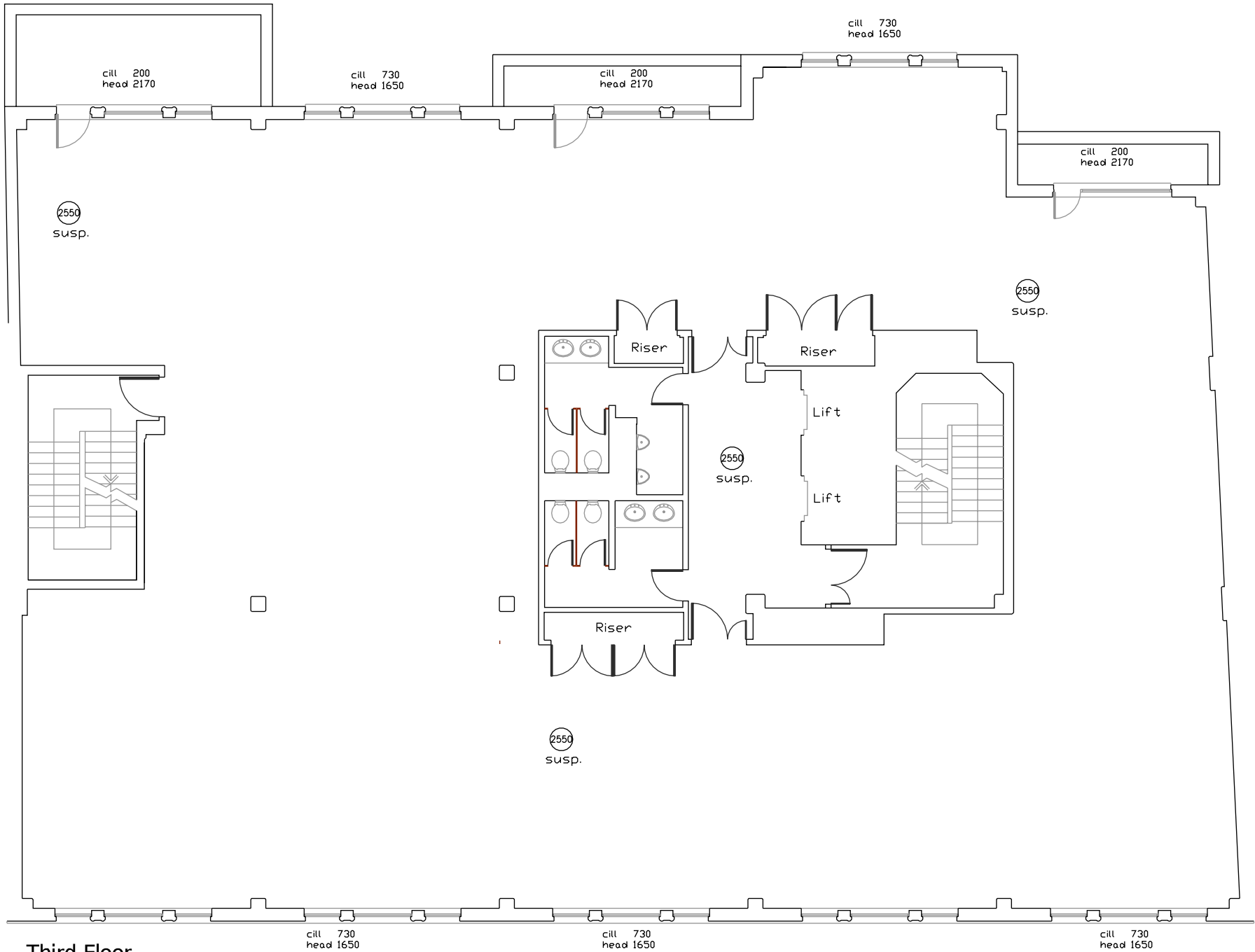
Third Floor
